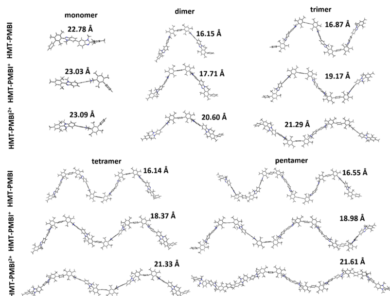
Figure 2. Effect of charge on the conformations of various studied systems in the gas phase. Numbers represent the normalized end-to-end distance values.
