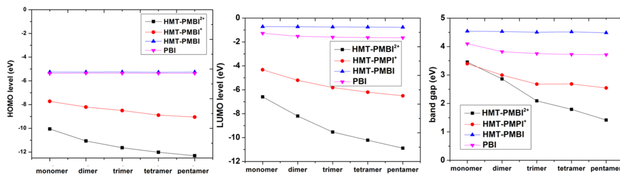
Figure 4. HOMO, LUMO, and band gap of the studied polybenzimidazole-based ionenes.
